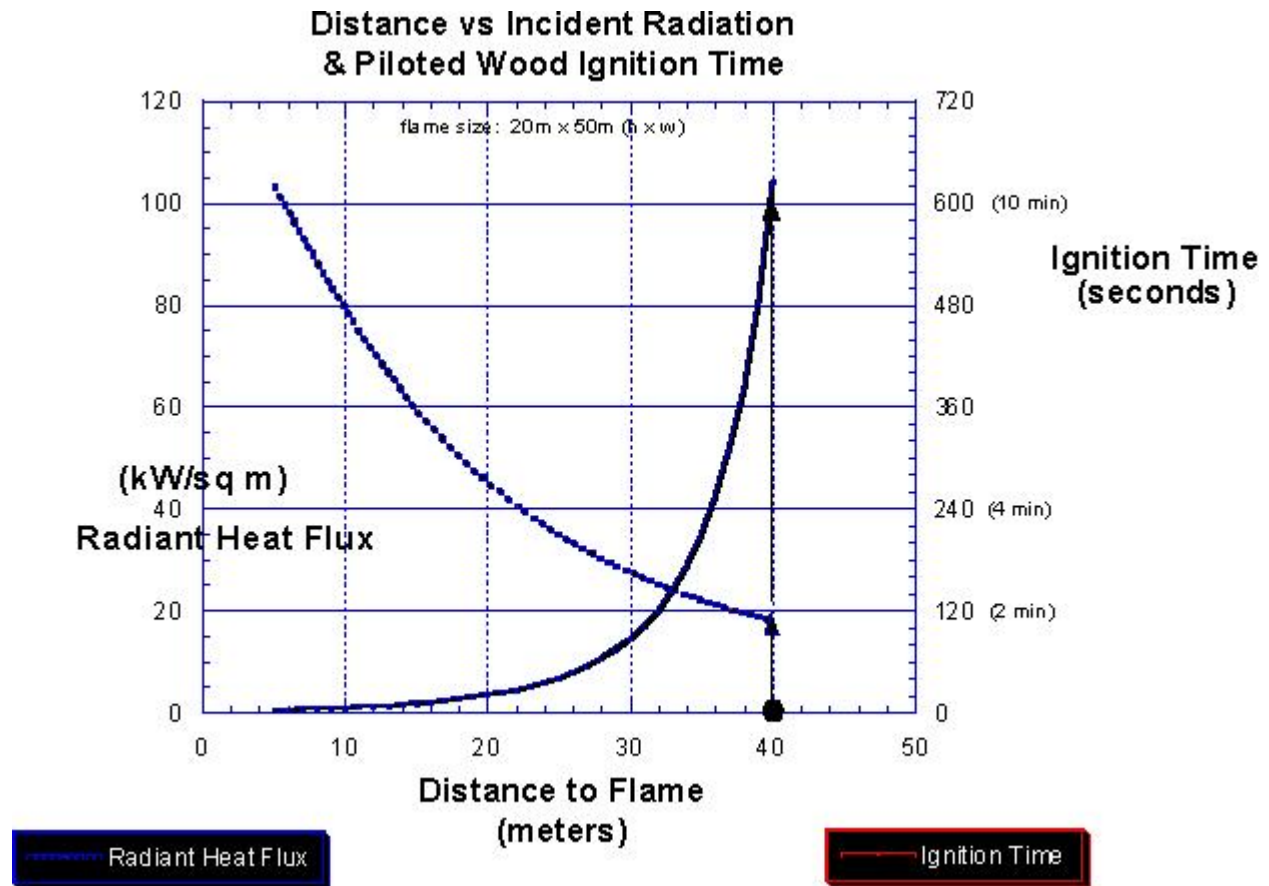
Figure 1-- SIAM calculates the incident radiant heat flux (energy/unit-area/time reaching a surface) and the minimum time for piloted ignition (ignition with a small ignition flame or spark) as a function of distance for the given flame size. The flame is assumed to be a uniform, parallel plane, black body emitter.
